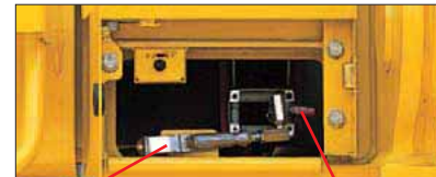
Grease gun The grease gun can be reached from ground level.
